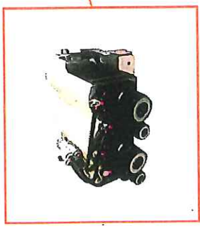
Standard Four Cross Milling Stations 2x ER16 & 2x ER11 for Increased Productivity
